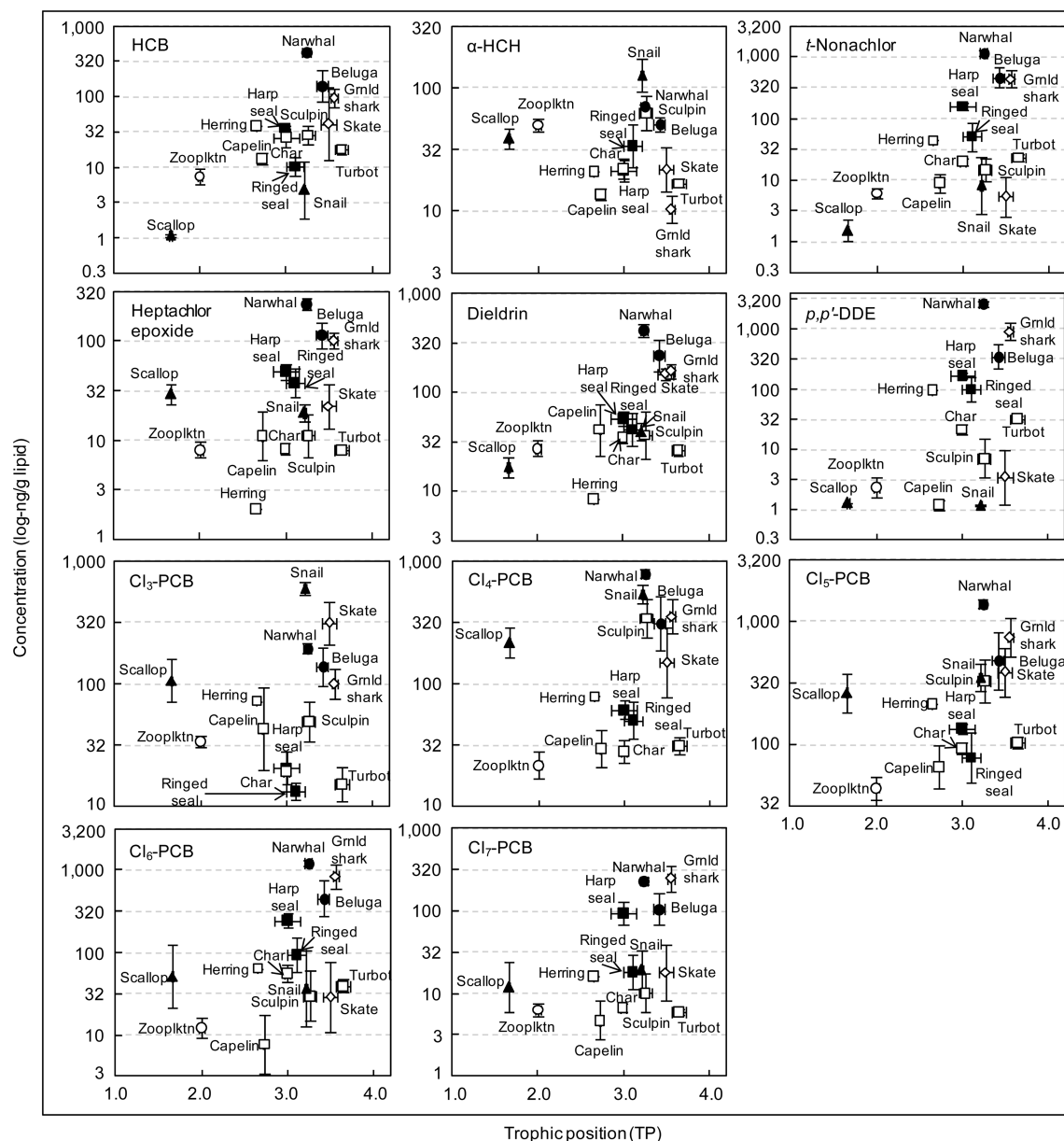
Figure 2. Contaminant concentration versus trophic position (TP) for zooplankton (○; zooplktn), benthic invertebrates (▲; scallop, snail), teleost fishes (□; herring, capelin, char, sculpin, turbot), elasmobranch fishes (◇; skate, Greenland shark (Grnld shark)), pinnipeds (■; harp seal, ringed seal) and cetaceans (●; beluga whale, narwhal) from the Cumberland Sound food web sampled in 2007–2008.
